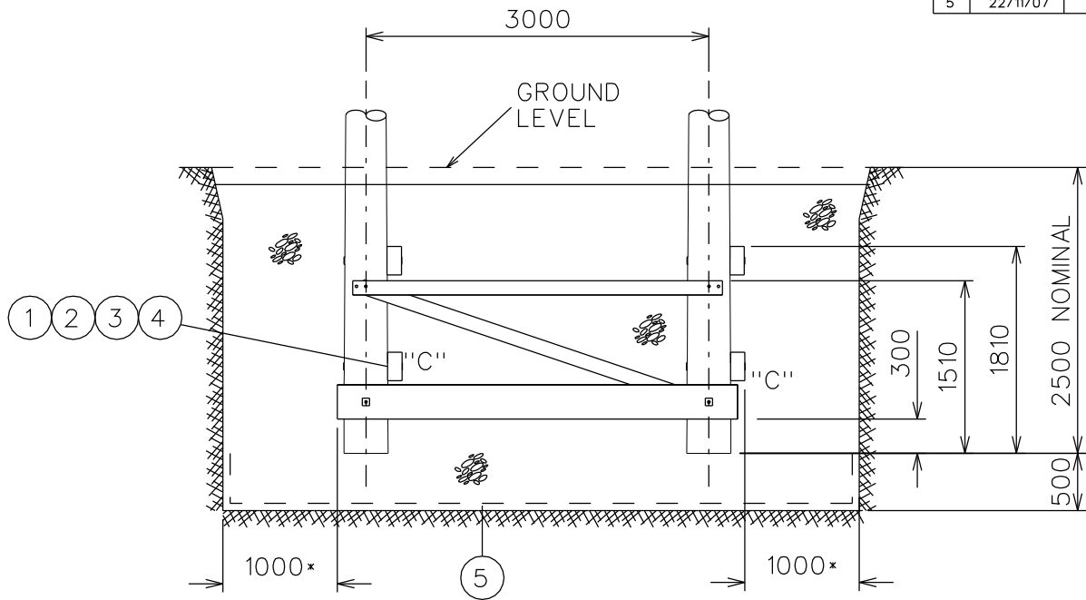
14M POLE FRONT ELEVATION
